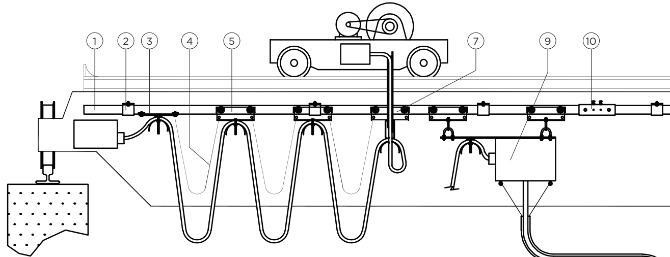
Item 6 Cable length = track length + 10% + 2 tails at V - up to 40 m/min. Item 5 Carrier quantity is to be based on system length + loop depth.
